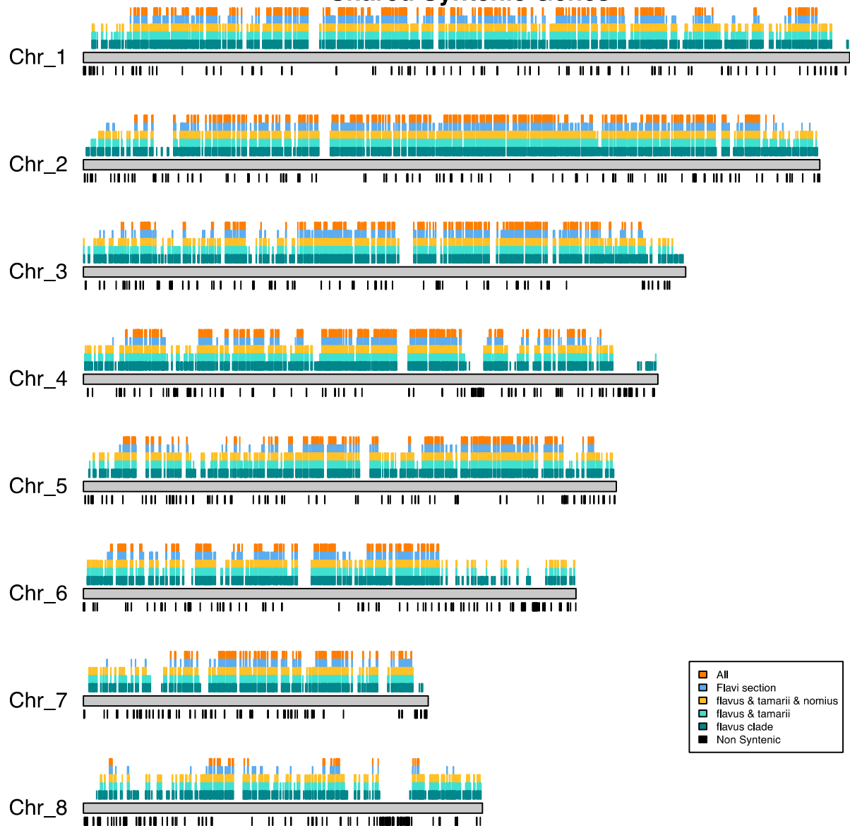
Supplementary Figure 6 - Syntenic genes mapped to the A. oryzae genome. The grey bars represent the A. oryzae genome. Syntenic genes were found using A. oryzae as reference comparing all the other species to this genome. Above the chromosomes syntenic genes shared with all species in a certain group is shown. Dark turquoise - A. flavus clade; light turquoise - A. flavus and A. tamaris clade; yellow - A. flavus , A. tamaris and A. nomius clade; blue - Flavi section; orange - Flavi section, A. nidulans and A. fumigatus . Below the chromosome the non-syntenic genes, found to be non-syntenic in all the species, are shown in black.
